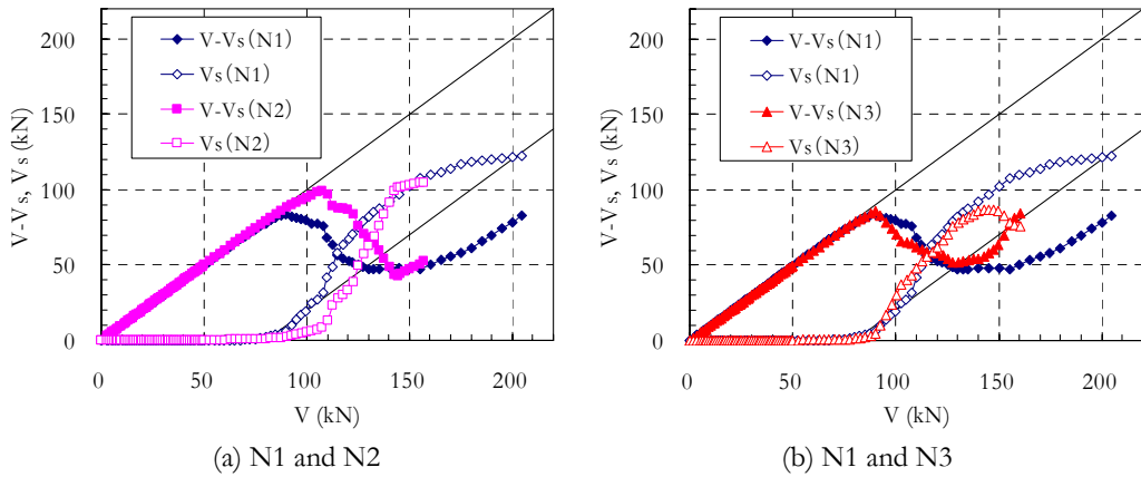
Figure 5: Comparisons of the shear strength contributions by concrete and stirrups
