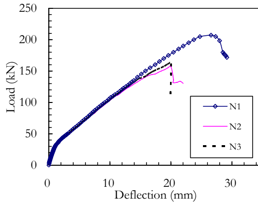
Figure 3: Load-deflection curve
