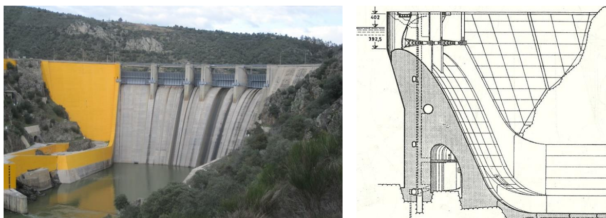
Figure 1.1: Bemposta dam. General view and central vertical cross-section
