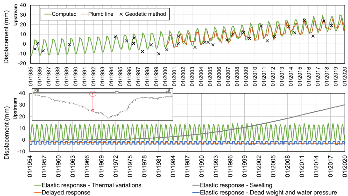
Figure 3.11: Radial displacement measured by the plumb line 2 and by geodetic methods and computed by the structural model
