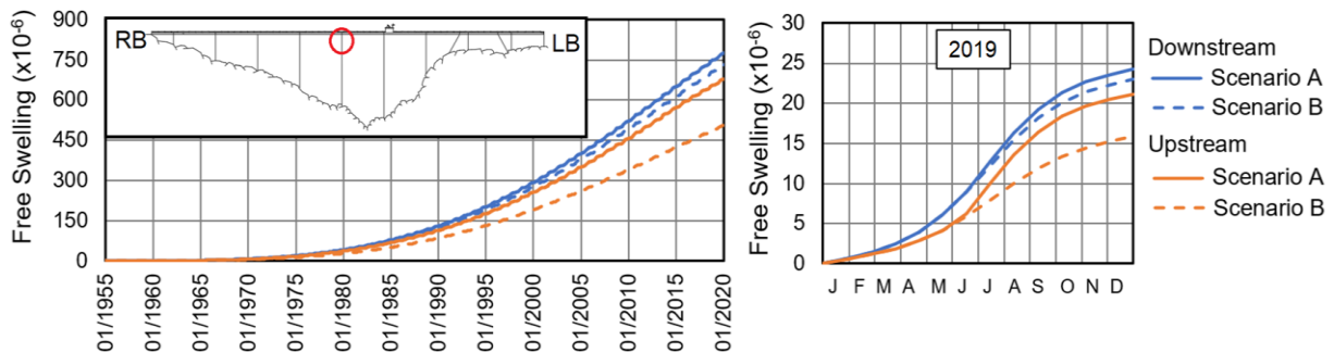
Figure 3.15: Free swelling evolution at the point at elevation 1651.0 m of joint E (upstream and downstream), for scenarios A and B, from the first filling of the reservoir to the end of 2019 (on the left) and during 2019 (on the right)
